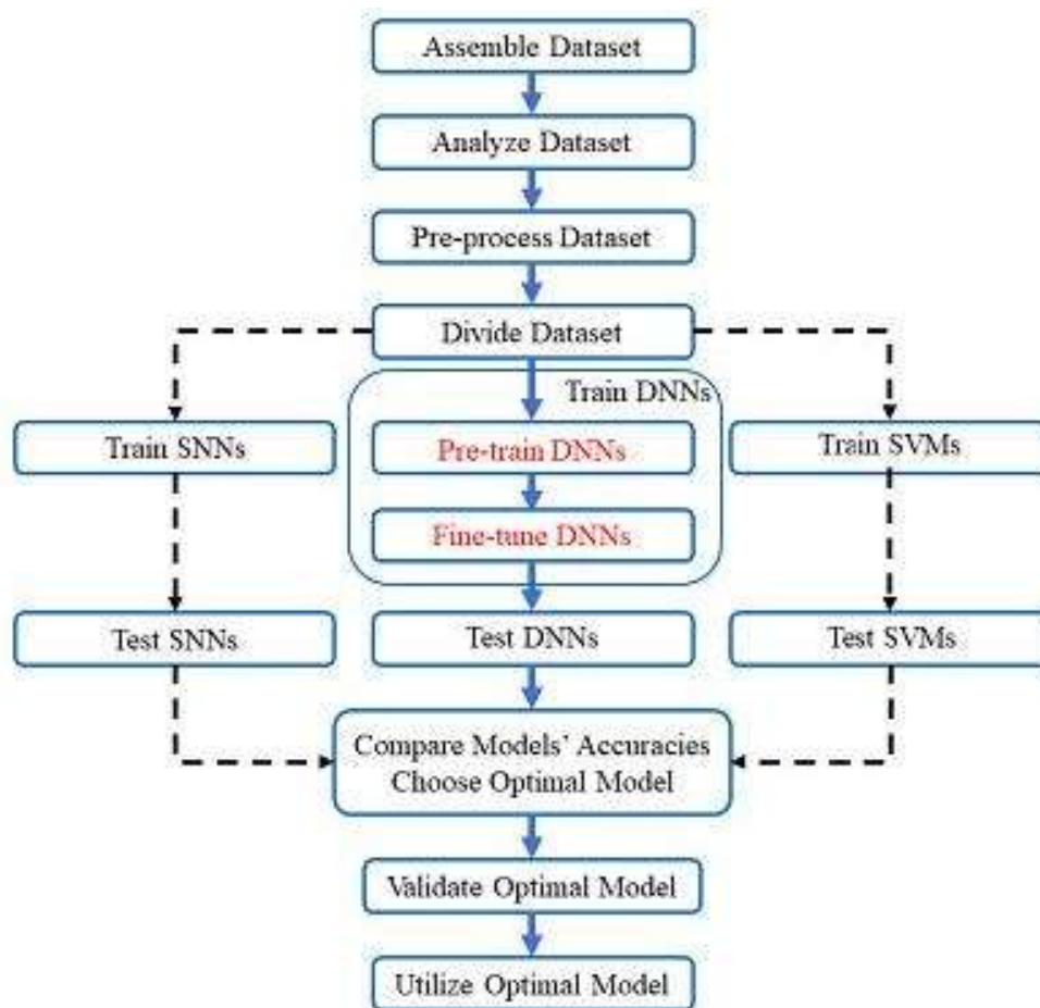
Figure 1: ANN algorithm
